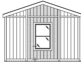
OPT. UPGRADED HITCH END ELEVATION/ FRONT ENDWALL
